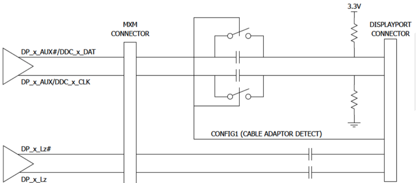
Figure 12.1 Dual-mode DisplayPort Implementation
