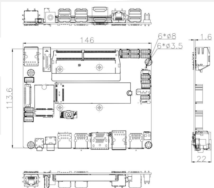
Mechanical Drawing (TOP Side)
