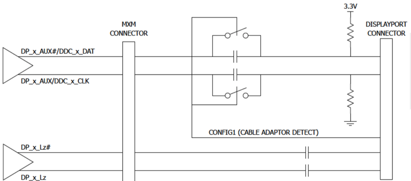
Figure 11.1 Dual-mode DisplayPort Implementation
