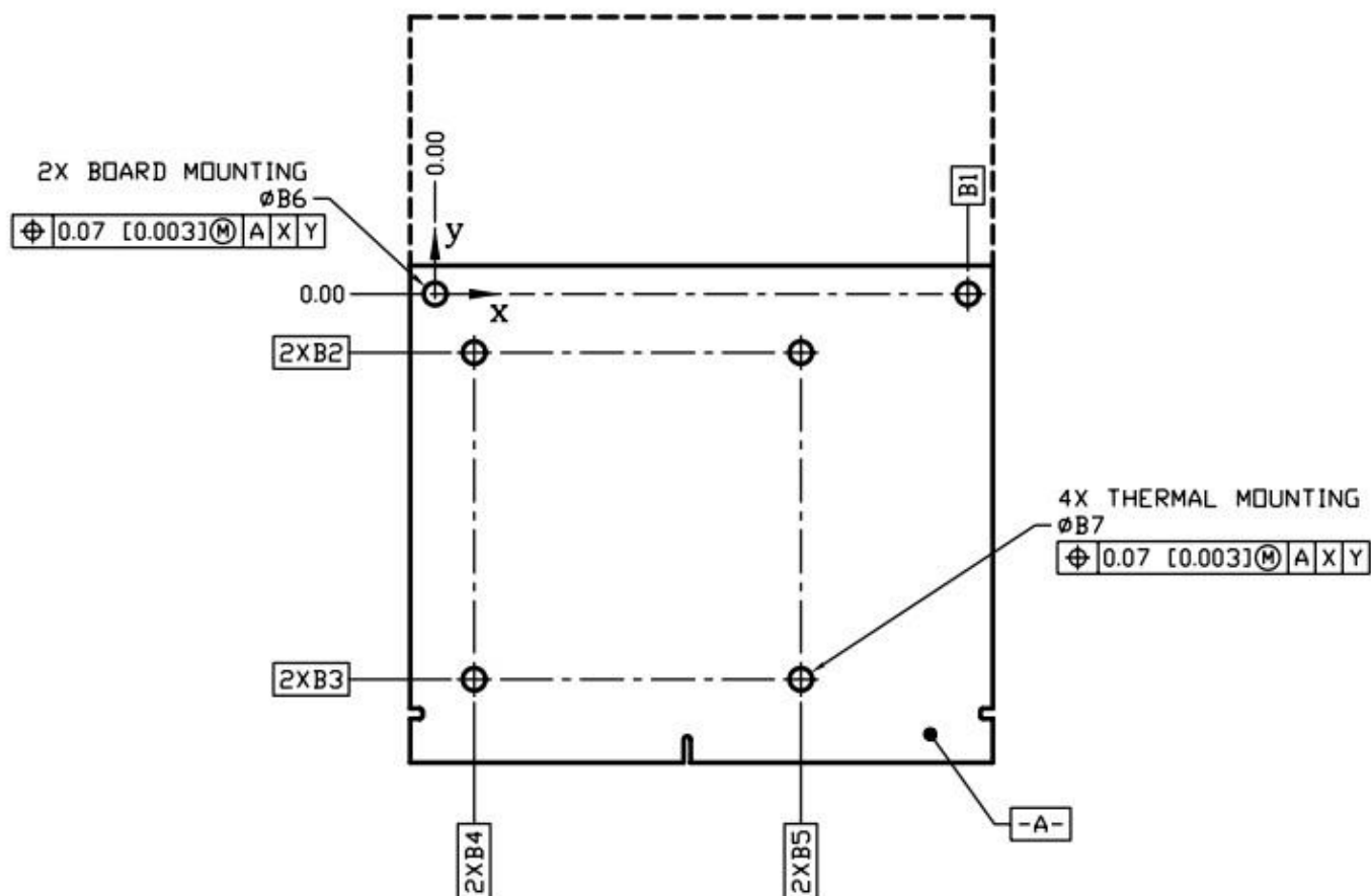
Figure 4.1: Mounting Holes
