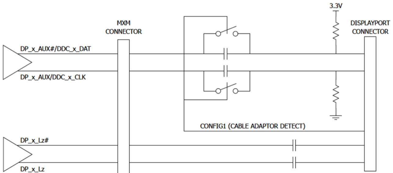
Figure 7.1 Dual-mode DisplayPort Implementation
