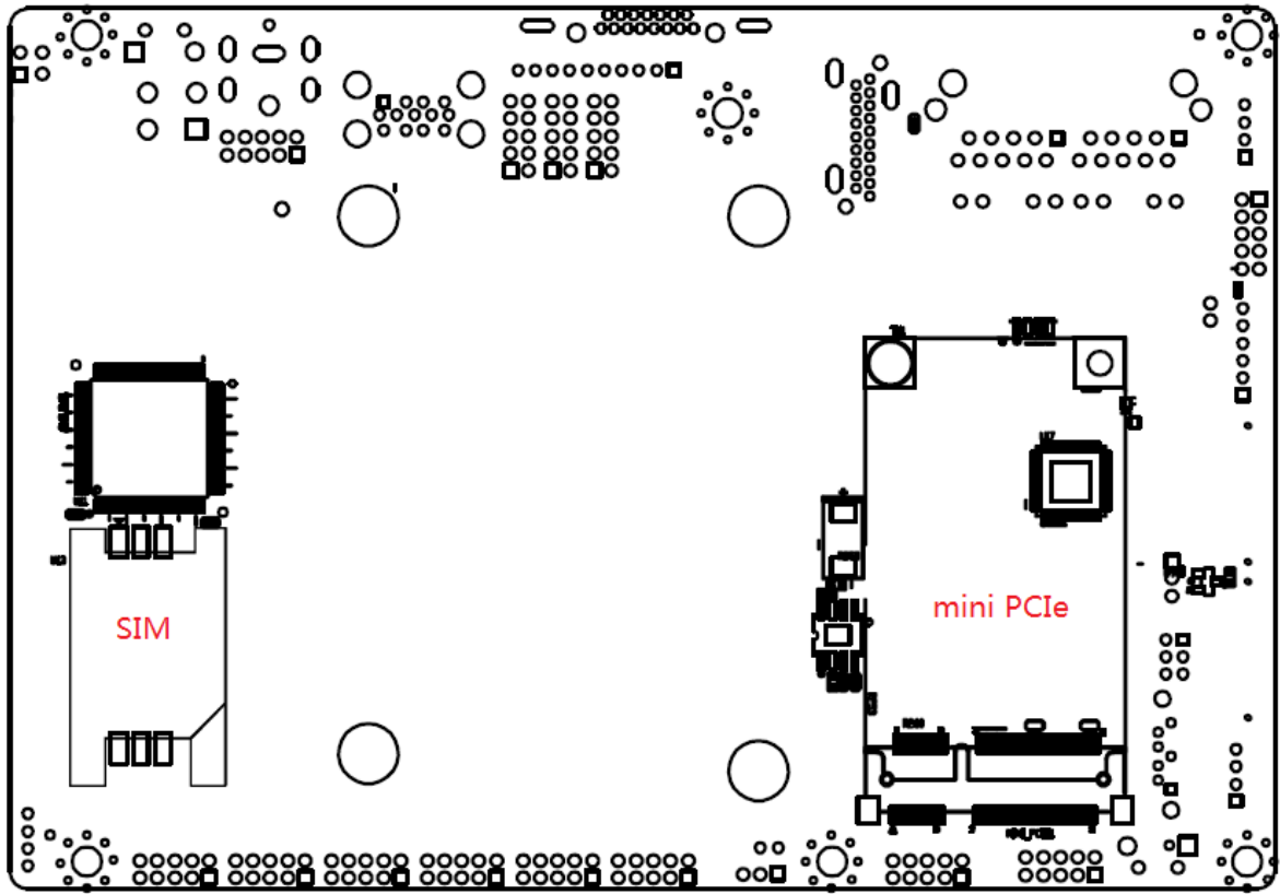
BOTTOM VIEW
