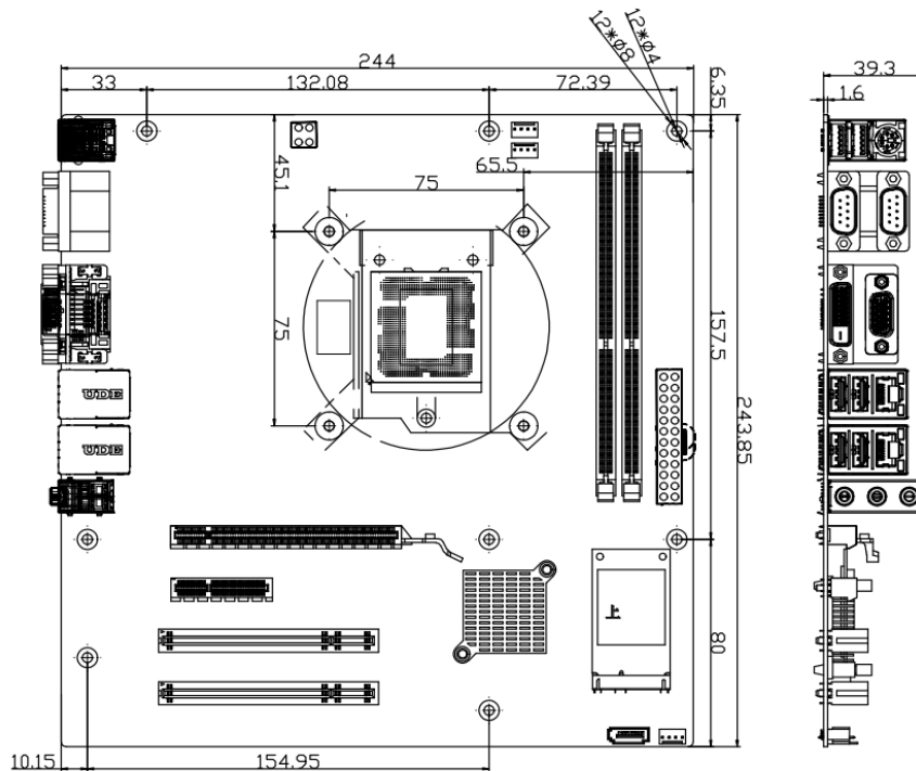
Mechanical Drawing (TOP Side)
