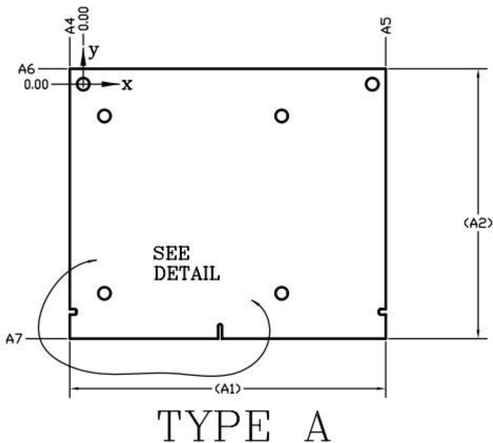
Figure 2.1: Board Outlines
