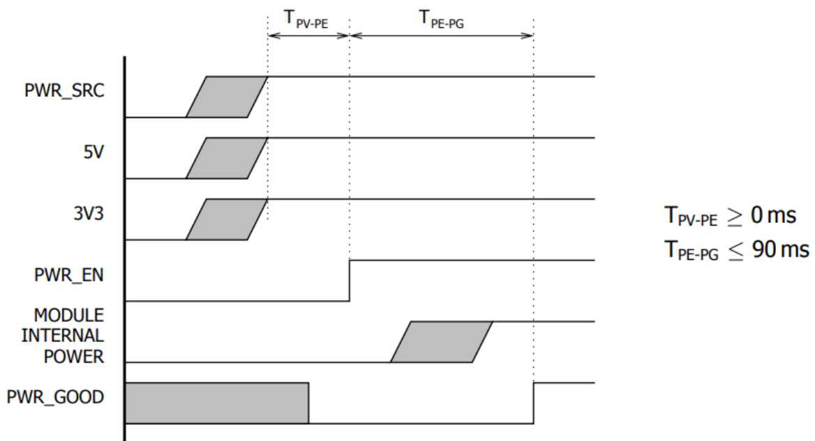
Figure 7.1 Power Sequencing
