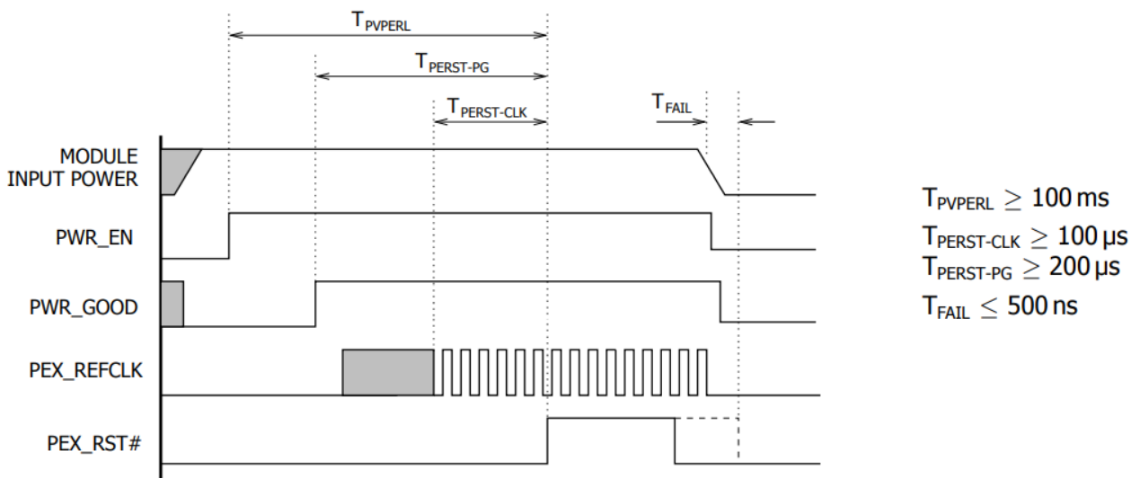
Figure 9.1 Reset Sequencing
