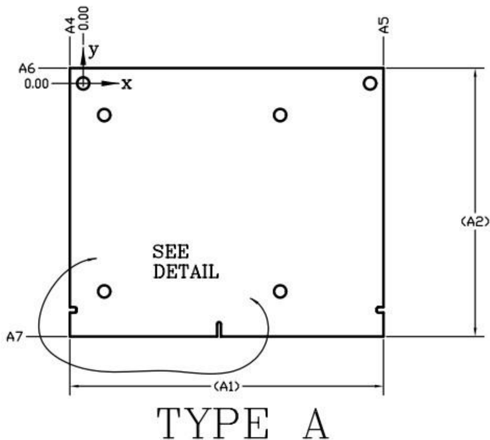
Figure 2.1: Board Outlines
