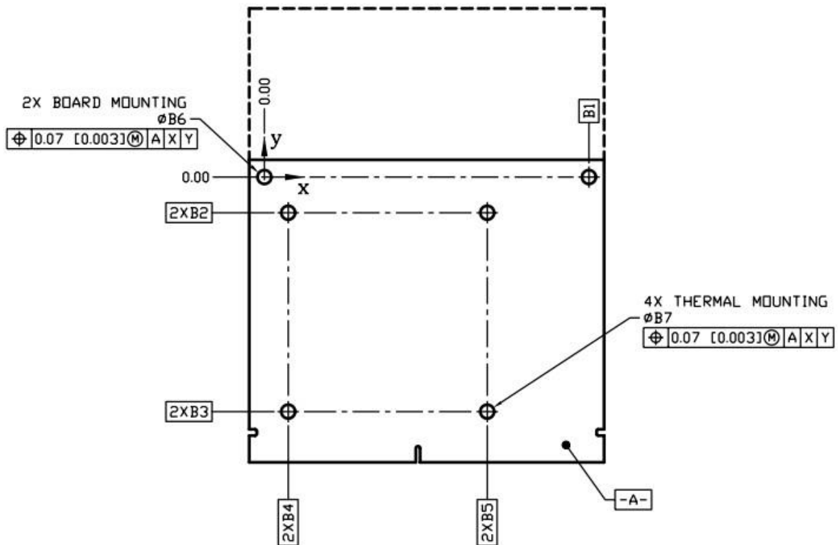
Figure 3.1: Mounting Holes
