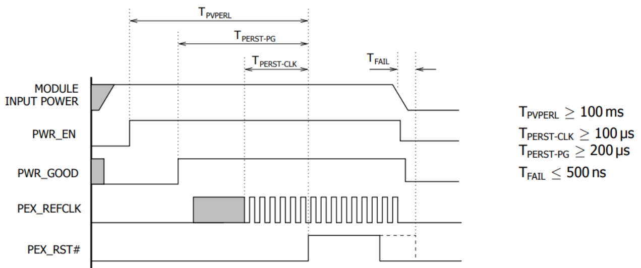
Figure 9.1 Reset Sequencing
