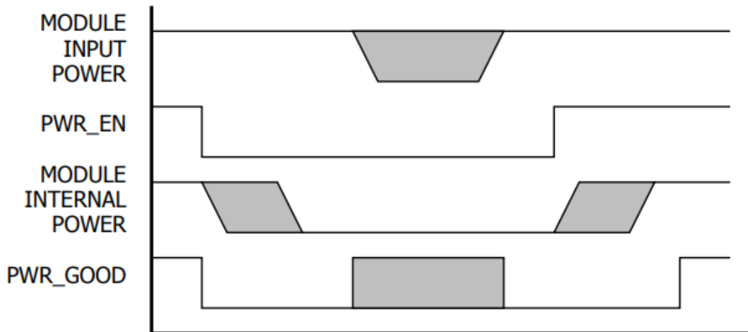
Figure 8.1 Module Power Down
