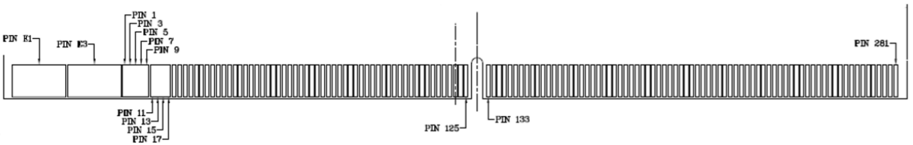
Figure 5.2 MXM Connector (Card Bottom)
