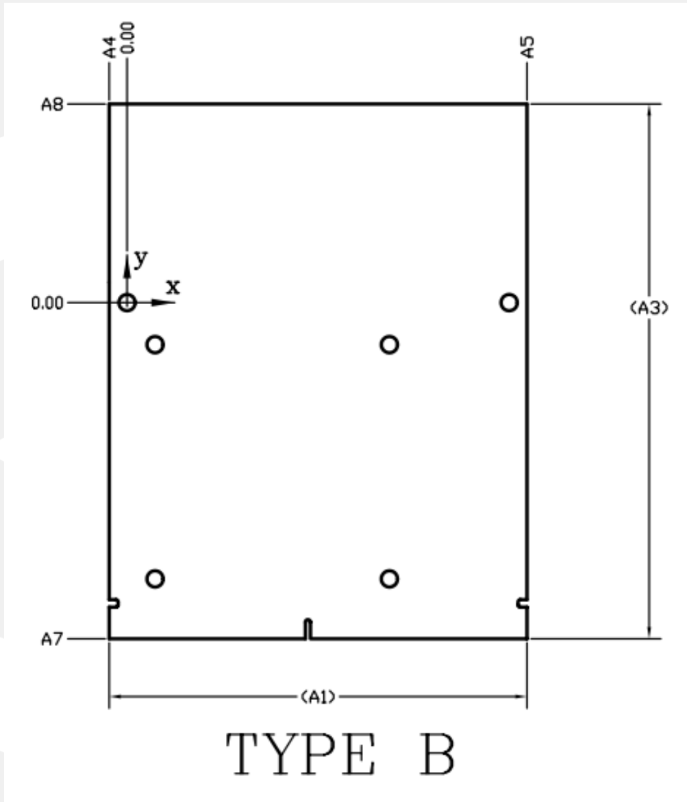
Figure 3.1 Board Outlines
