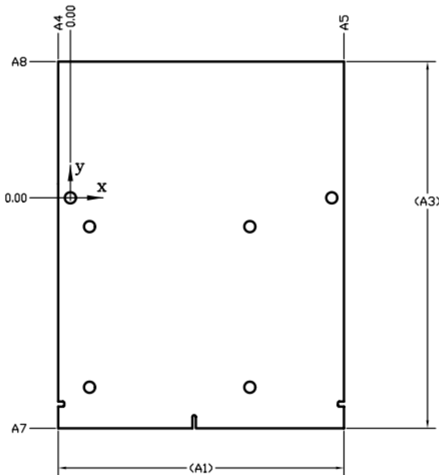
Figure 3.1 Board Outlines
