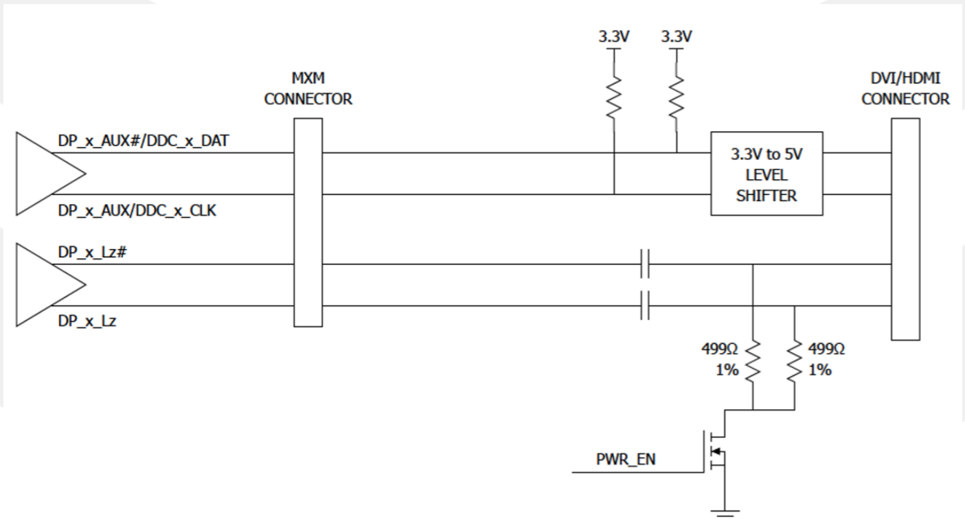
Figure 12.1 DVI/HDMI Implementation Using DP Interface
