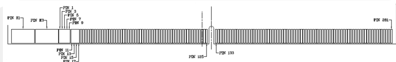
Figure 7.2 MXM Connector (Card Bottom)
