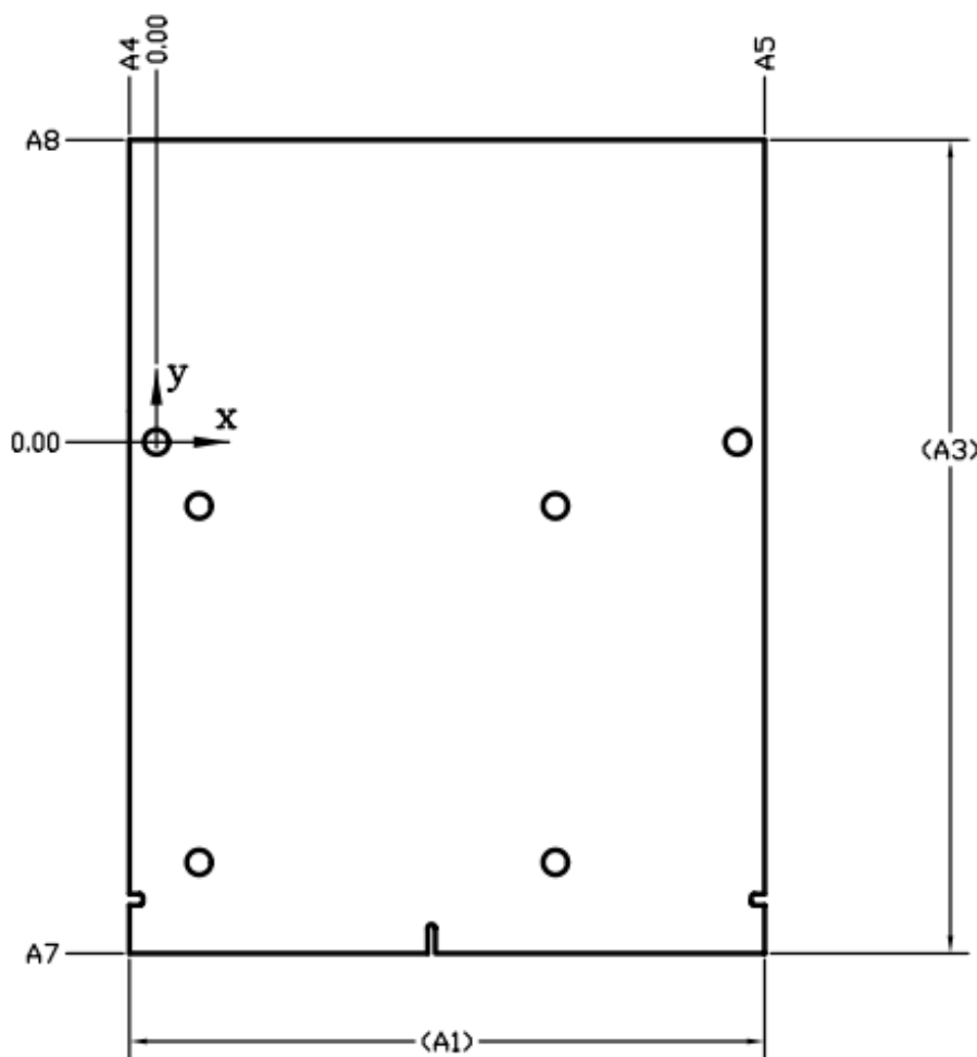
Figure 4.1 Board Outlines
